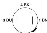
Pin assignment for QUICKON connection, 3-pos.
