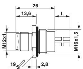
Dimensions: plug, front mounting
