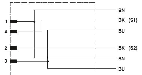
Contact assignment of the M8 Y connector
